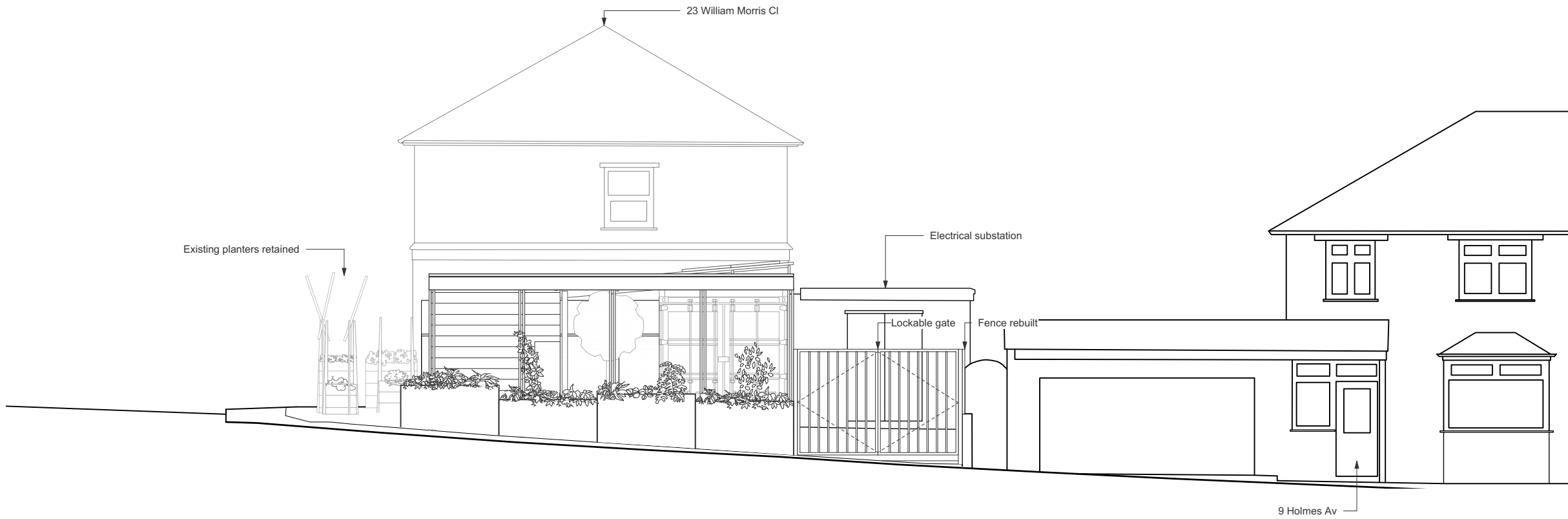
Existing Elevation A
